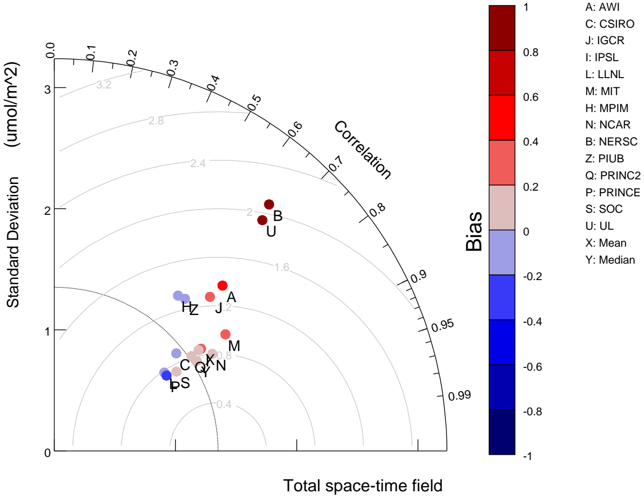
CFC-11 inventory Taylor diagram
